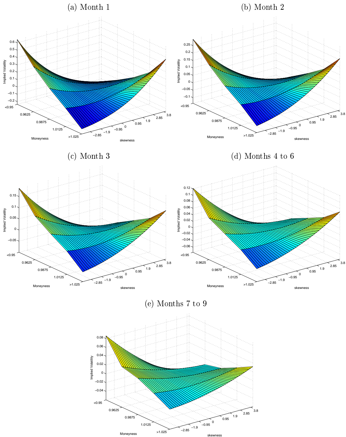
Figure 5: Deviations of implied volatility and skewness surfaces from the BSM IV values for different maturity categories. Moneyness is defined as \ln(S/K)(-r\tau) and maturity groups are defined using settlement dates.
